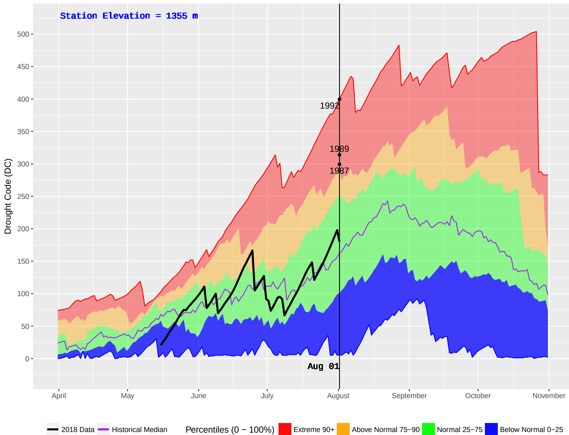
BIG VALLEY (262) : Historical (1987–2016) and Current (2018) Daily Drought Code (DC)
