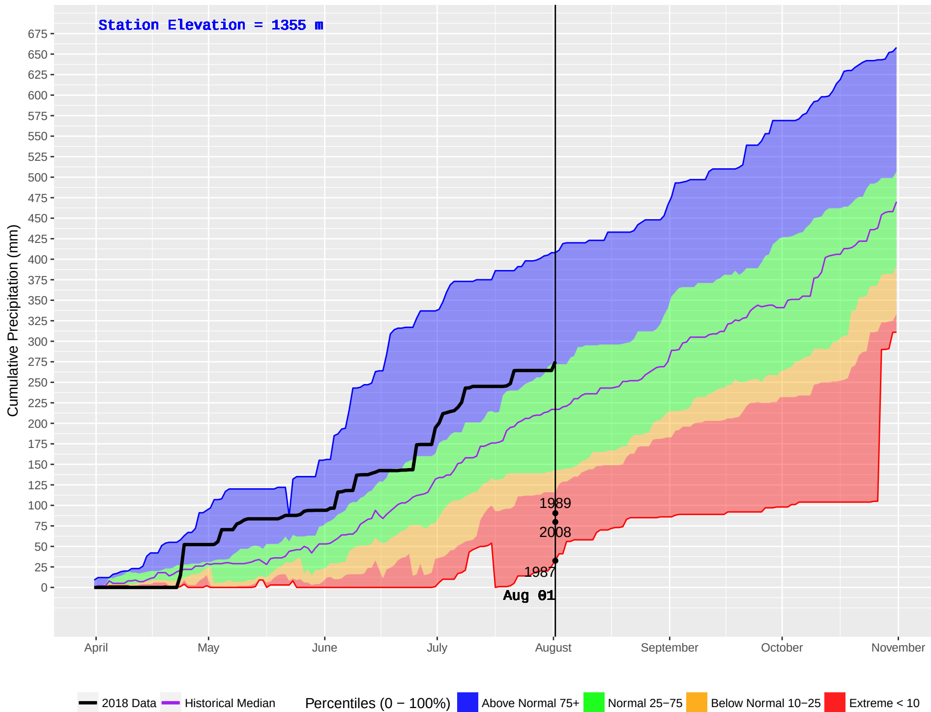
BIG VALLEY (262) : Historical (1987–2016) and Current (2018) Daily Cumulative Precipitation
